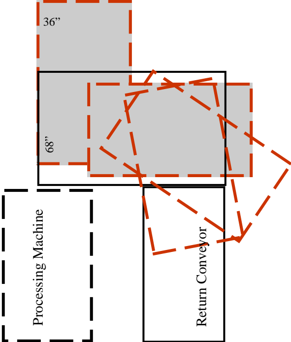
PB 48L x 72W w/30" Rollers Maximum part size is 36" x 68"
