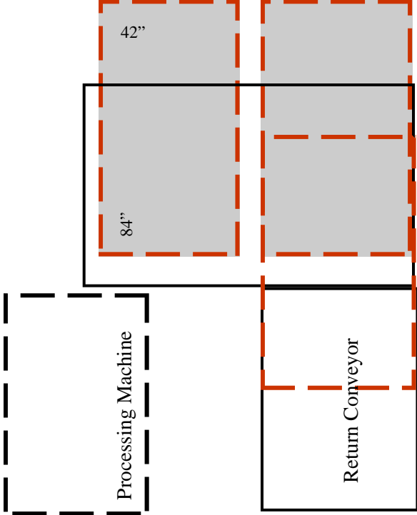
TB 60L x 96W w/36" Rollers Maximum part size is 42" x 84"
