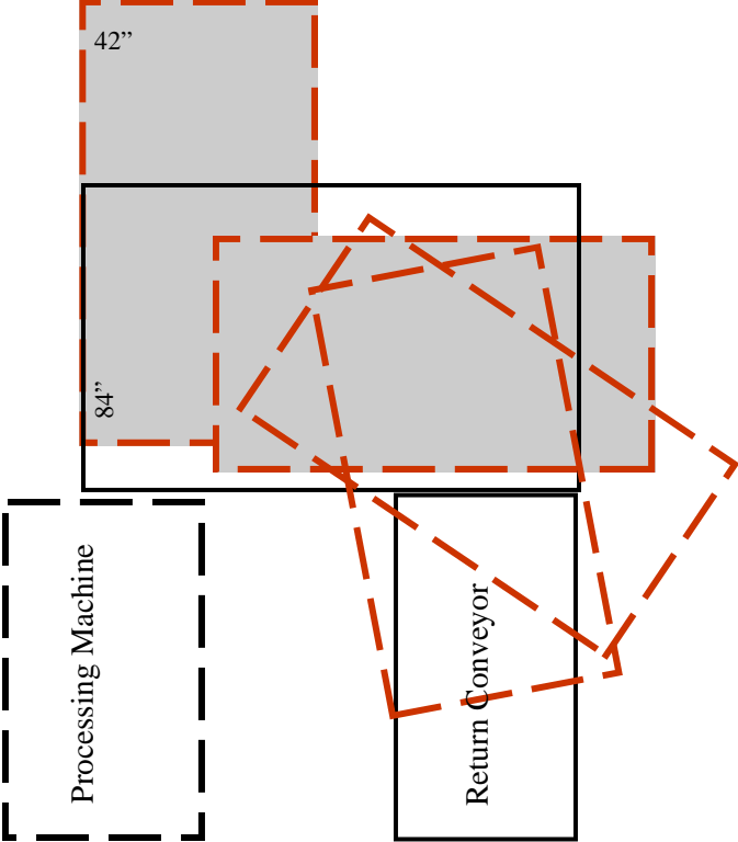
TB 60L x 96W w/36" Rollers Maximum part size is 42" x 84"
